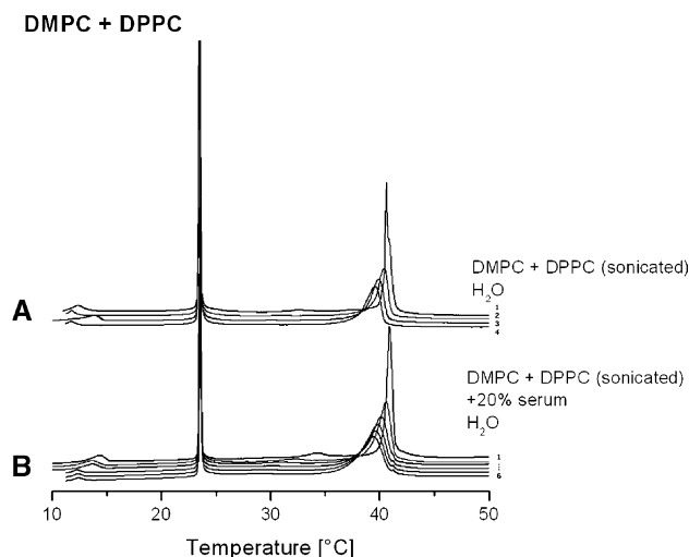
Fig. 5. Consecutive heating thermograms of mixtures of DMPC and DPPC sonicated dispersions, prepared separately, mixed extempore at 5 °C at equimolar lipid ratio, immediately filled into the calorimetric cell at that temperature and scanned at 30 °C/h between 5 and 50 °C (thus, 3 h elapse between the onset of the sequential heating scans): (A) dispersions of DMPC and DPPC; (B) dispersions of DMPC and DPPC with 20 vol.% serum.
